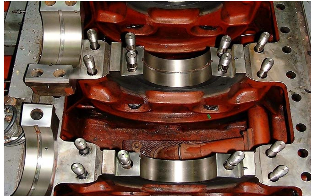
Completed Main Bearing Pockets And Caps After Capping With Nickel
