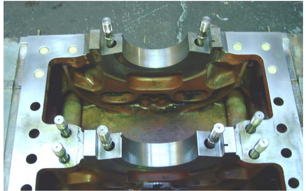
Completed Repair Of The Fretted Face After Capping With Nickel
