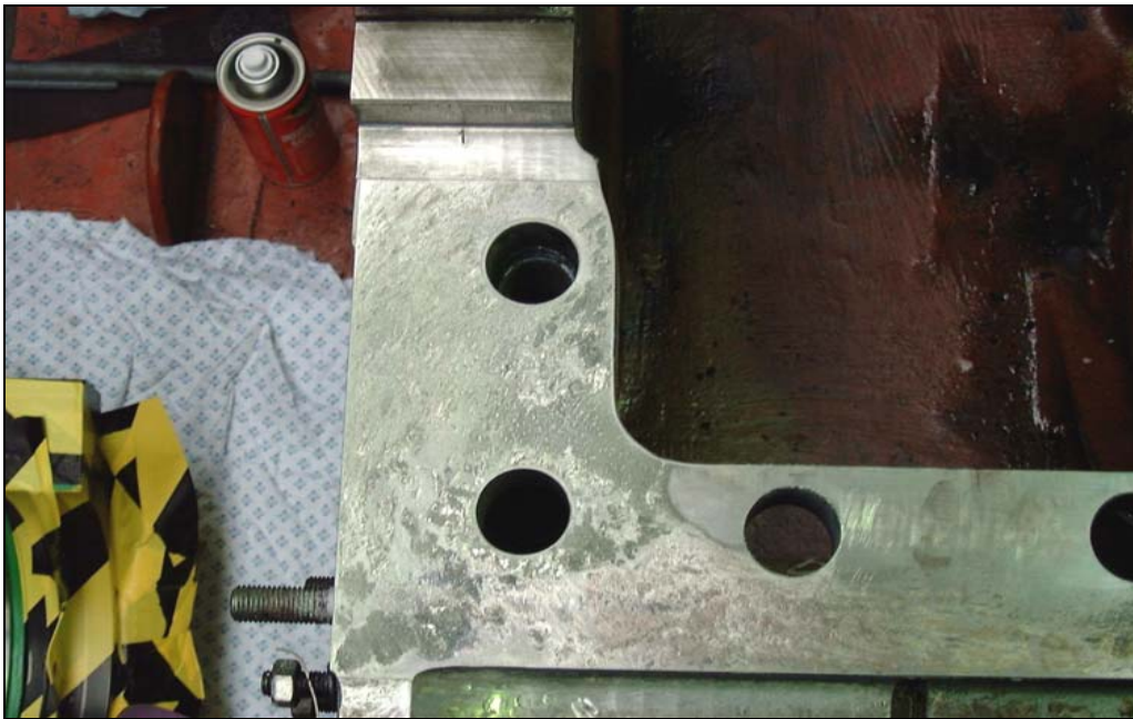
Badly Fretted Bedplate Mating Face
