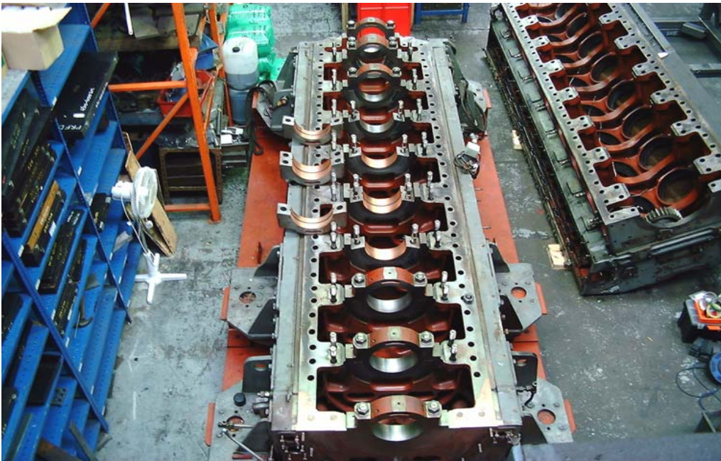
Plated And Line Bored Main Bearing Pockets And Caps
