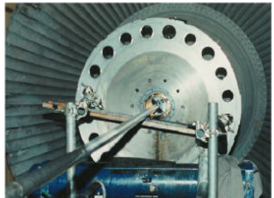
Internal Honing of a 110 mm Ø 4 Metre long Turbine Rotor Bore
