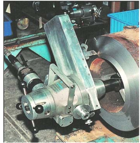
An end prep being carried out on a thick wall tube using an I/D mount
