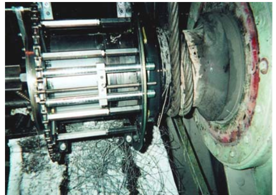
A 300mm \varnothing Fanshaft Journal During Machining
